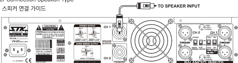
FIGURE4. Speaker Connection Speakon Type
