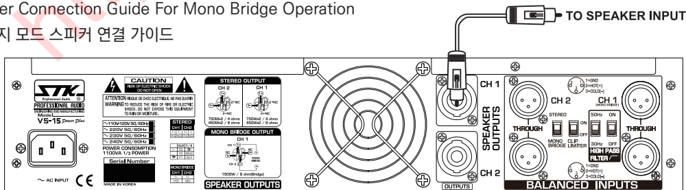
FIGURE4. Speaker Connection Speakon Type
